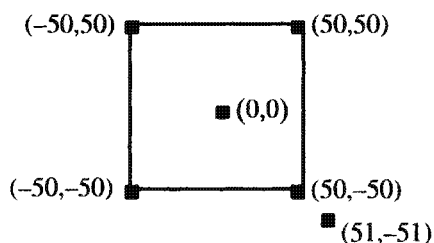
Fig 8.2. Layout of sample points relative to the target block
