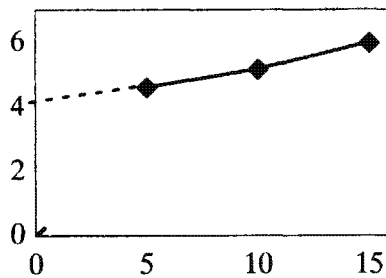
Fig. 4.3. Experimental variogram for samples spaced 5m apart. The solid line connects experimental values; the dotted one extrapolates back to the origin
