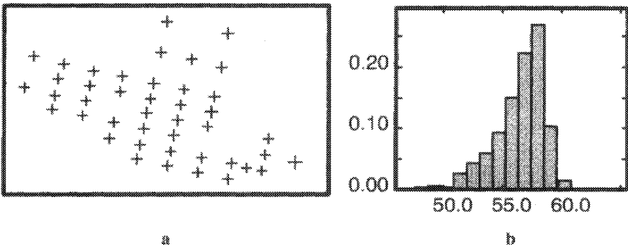
Fig 5.2. (a) Base map showing the layout of drillholes; (b) histogram of 485 Fe grades from 15m core sections. As is usual for iron ore, the grade histogram is negatively skew with a tail of small values to the left
