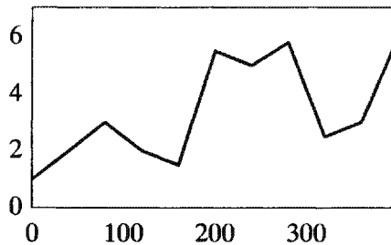
Fig 4.9. : Erratic saw tooth variogram
