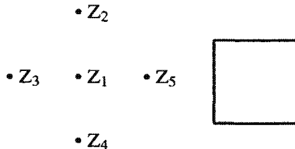
Fig 8.9. A symmetric data configuration with the block off center
