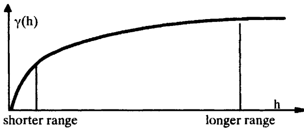
Fig 3.7. Nested structure composed of a short range structure and a longer one
