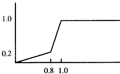
Non-standard variogram
