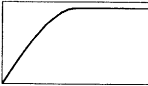
a Spherical Model
