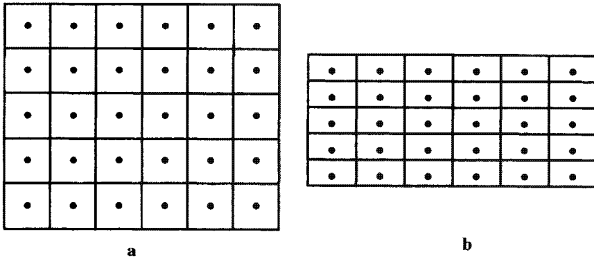
Fig. 10.3. (a) Original grid, (b) grid after taking account of anisotropy
